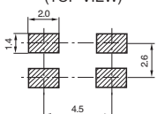
Reference land Patten (TOP VIEW)
